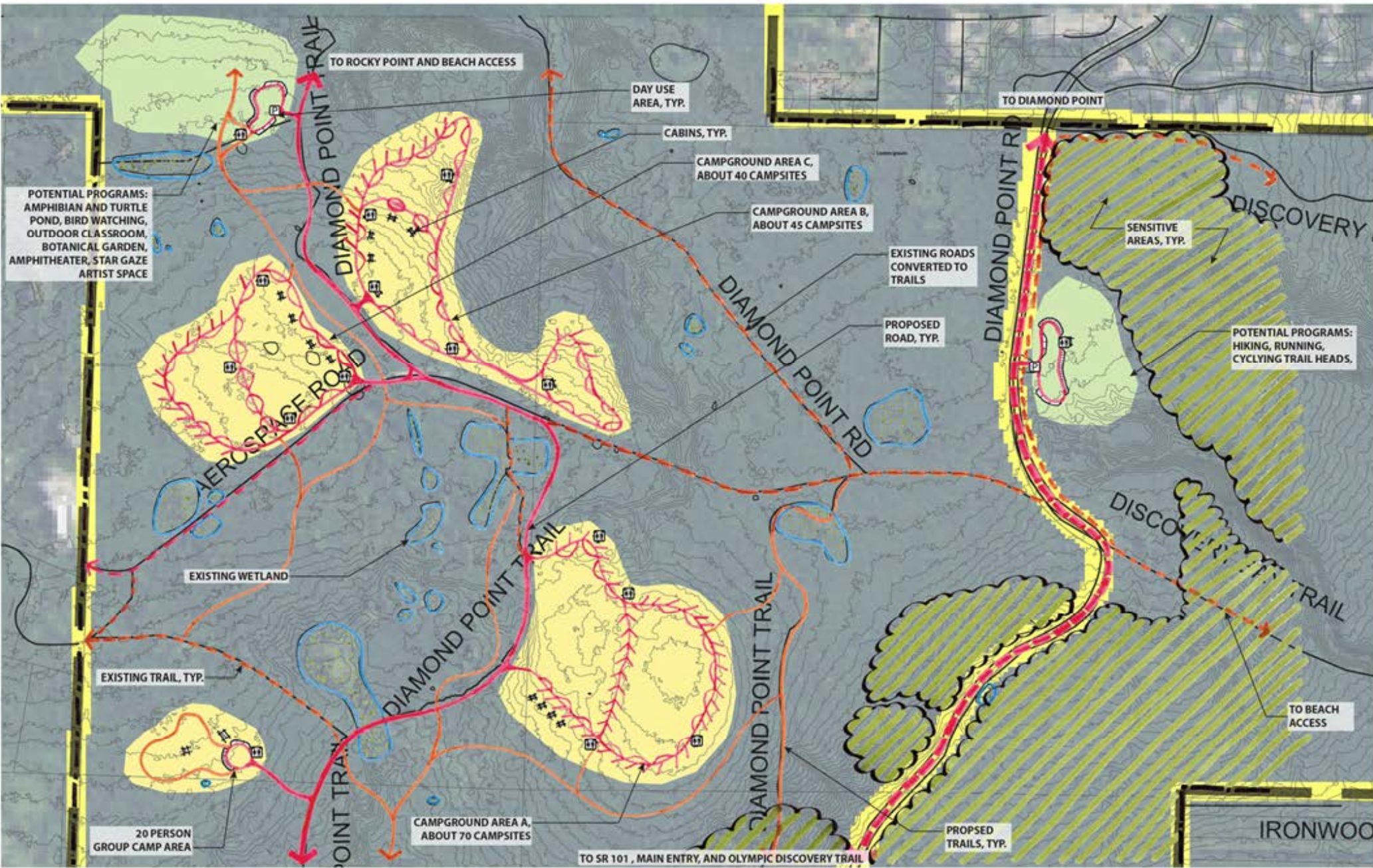
TRADITIONAL CAMPGROUND ALTERNATIVE (EXISTING TRAILS ONLY) CONCEPTUAL SITE PLAN
