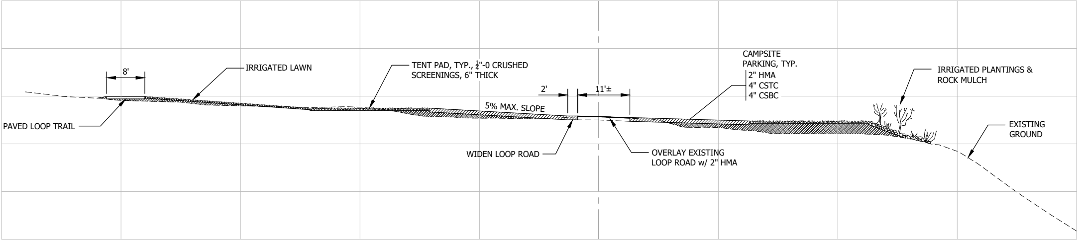
SECTION- 20+20
