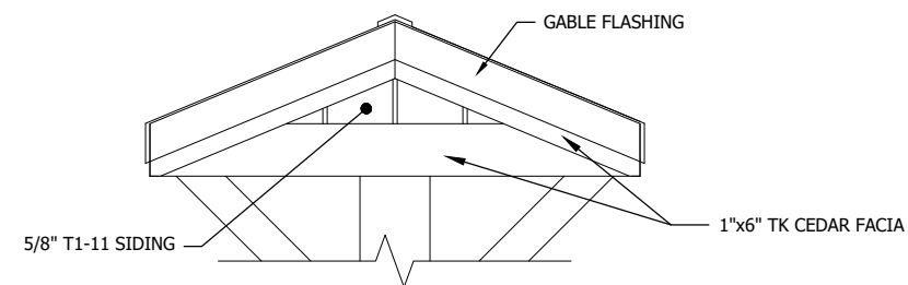
GABLE END ELEVATION
