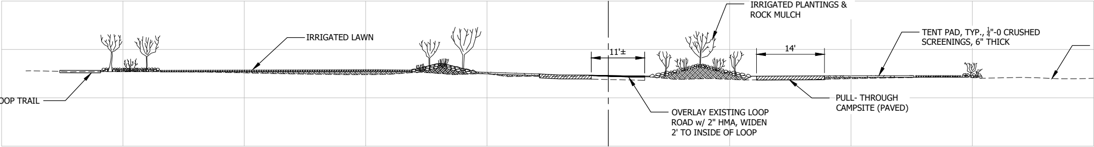
SECTION- 15+40
