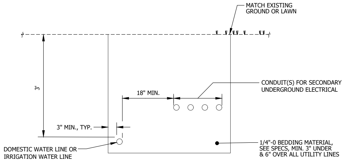
TYPICAL WATER / SECONDARY ELECTRICAL TRENCH N.T.S.
