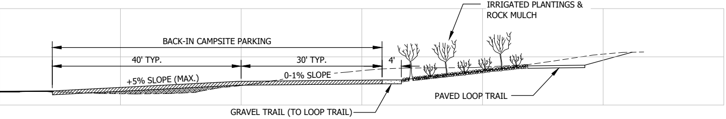
SECTION- CAMPSITE #14
